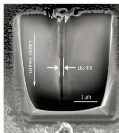
Nanodrilling in fused silica
