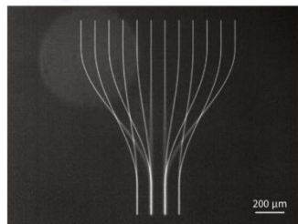
3D waveguide fabricated in fused silica glass.
